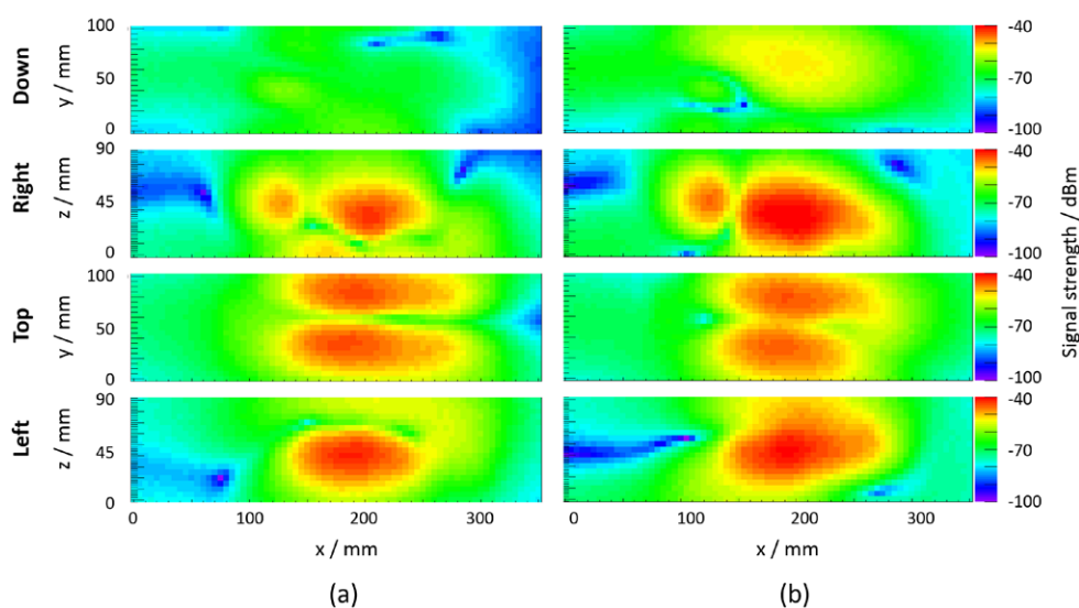
Figure 16. Field map measurement results ( y component of the emitted H field) for sensor die clocking with in-phase pattern (a) and checkerboard-phase pattern (b) at SDM level and a sensor die clock frequency of 127.78 MHz.
